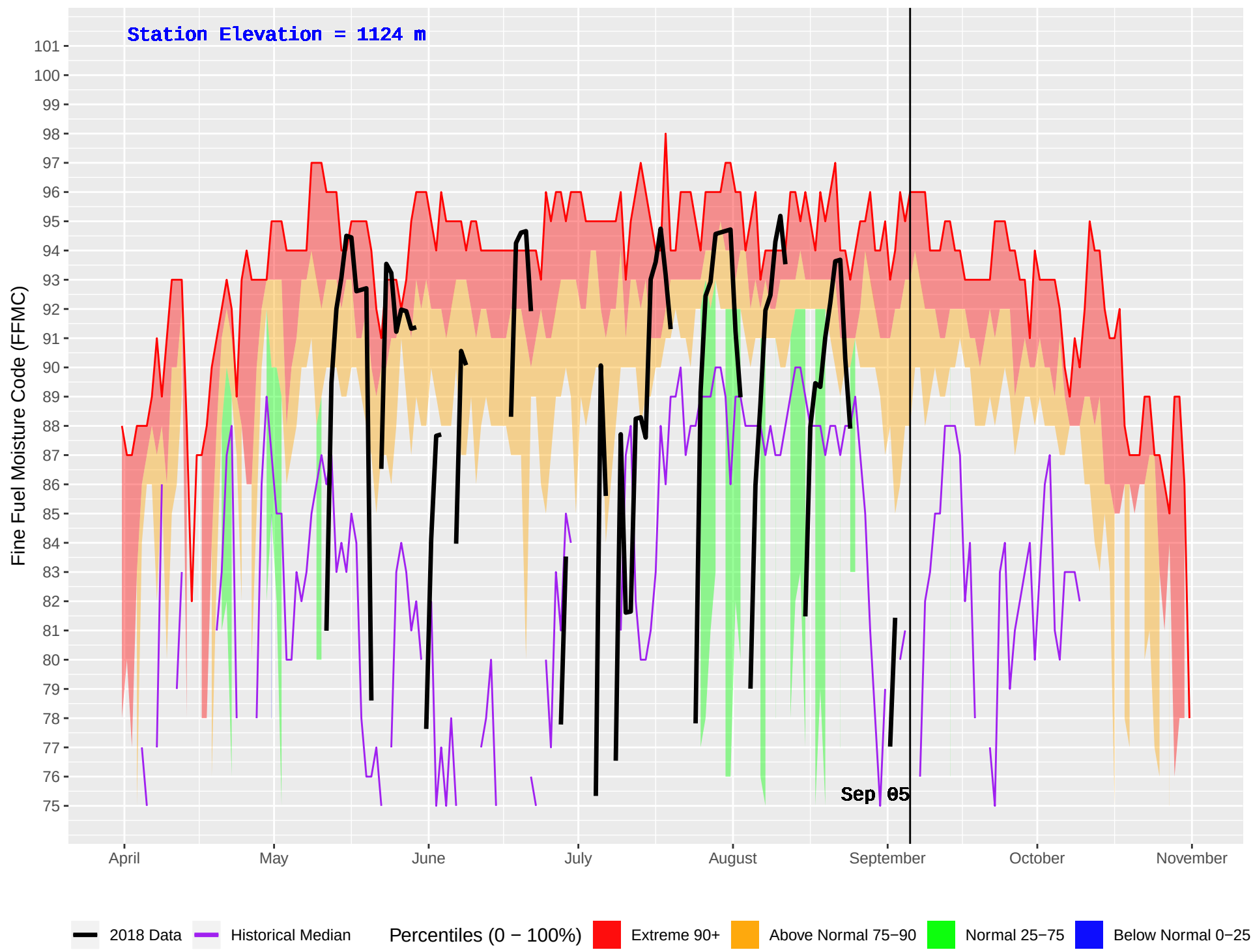
COLDSCAUR LAKE (232) : Historical (1979–2016) and Current (2018) Daily Fine Fuel Moisture Code (FFMC)
